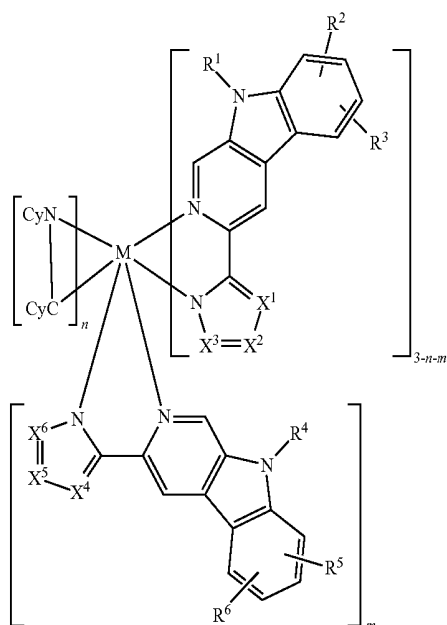
Chemical Formula 2
