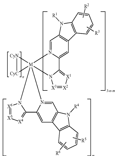
Chemical Formula 2
