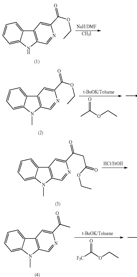
Reaction Scheme 1
