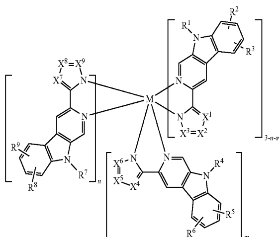
Chemical Formula 3
