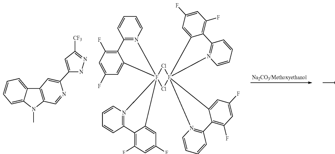
Reaction Scheme 2
